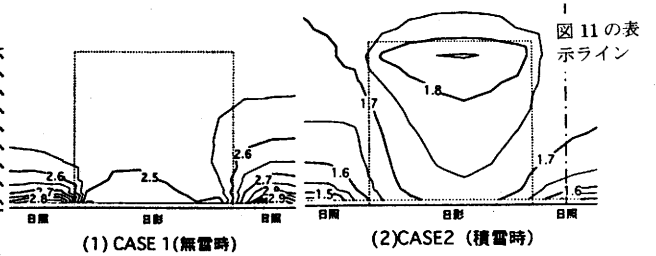
Fig.10 Distribution of air temperature (at lateral section)
