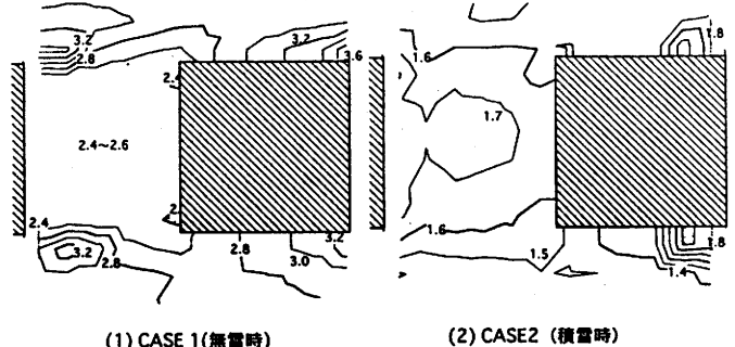
Fig.12 Distribution of air temperature (1m height)
