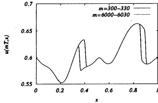
Fig. 4 u(mT, x) : T = 0.8 , L = 1000 , m=300, 301, \dots, 330 ( A = 0.5 , M = 0.6 )
