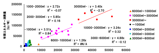
Fig. 5 Energy consumption of commercial buildings
